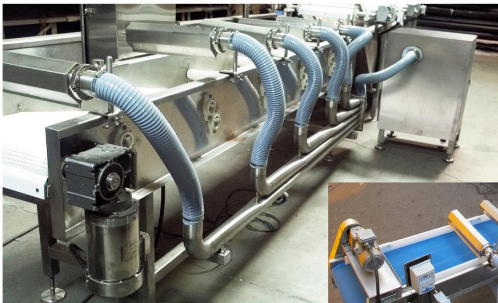
Air Knife Conveyor with Turnovers
